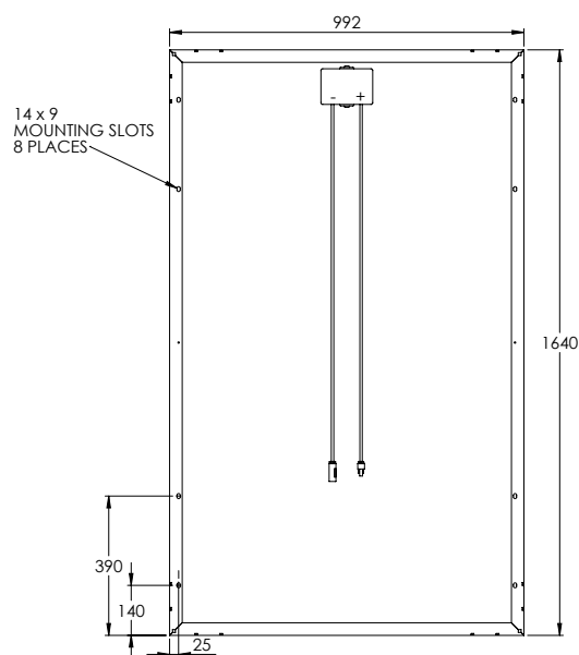
SG-240P6 Diagram
